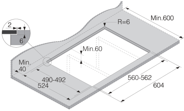
Flush-built
