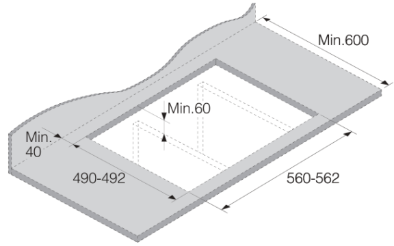
Top-built
